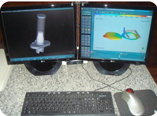
Software CAD-CAM
